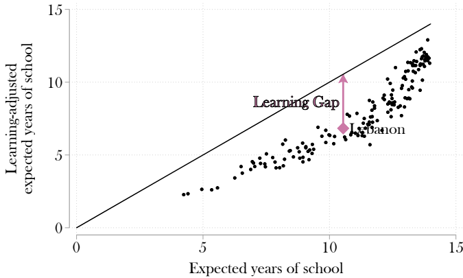
Figure 3. Learning Gap
