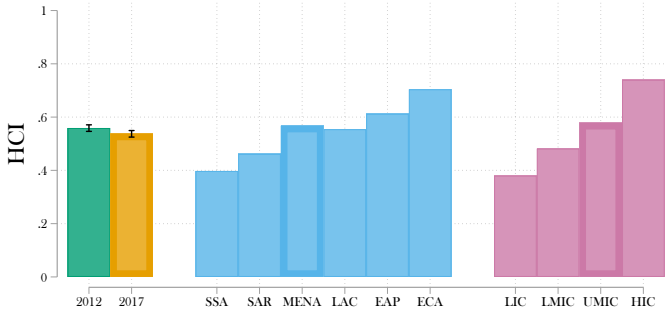
Figure 2. Benchmarking HCI
